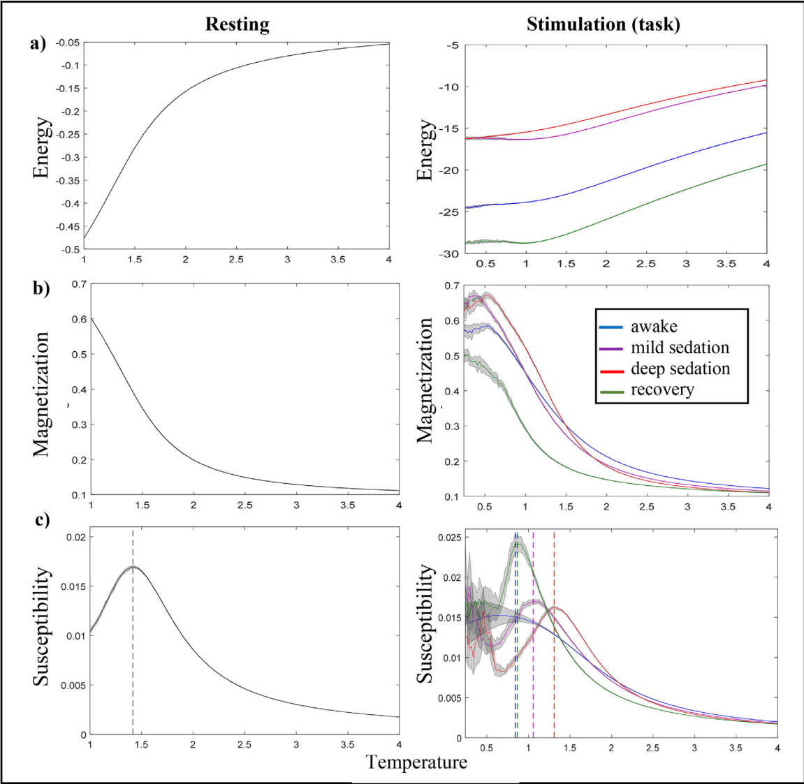
Fig. 2. Thermodynamic properties, a) Energy b) Magnetization c) Susceptibility calculated from the GIM during resting and under stimulation at four different levels of consciousness. The dashed lines represent the critical temperatures.
