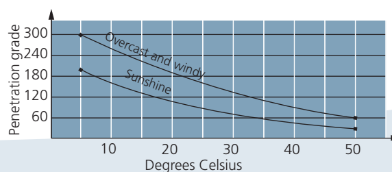
Fig. 3. Indication of suitable tack coat penetration grades for paving fabrics.
