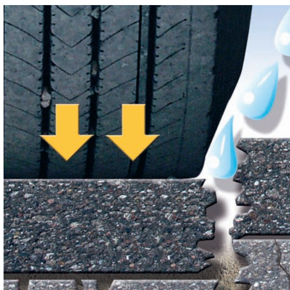
Fig. 2. Without paving fabric, reflective cracking of the new asphalt overlay will occur and surface water will enter the old asphalt layer. This will accelerate deterioration of the entire road construction.
