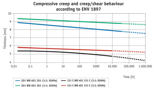
Fig. 2 Creep behaviour of Secudrain®
