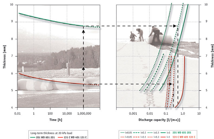
Fig. 1 Design chart to determine the water discharge capacity of Secudrain® WD as a function of the long-term thickness
