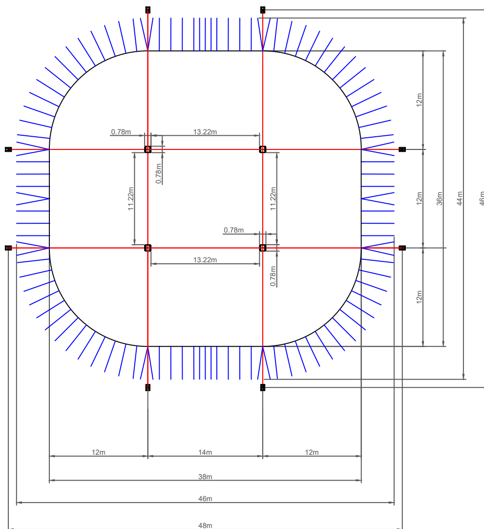
PLAN LAYOUT (NTS)
