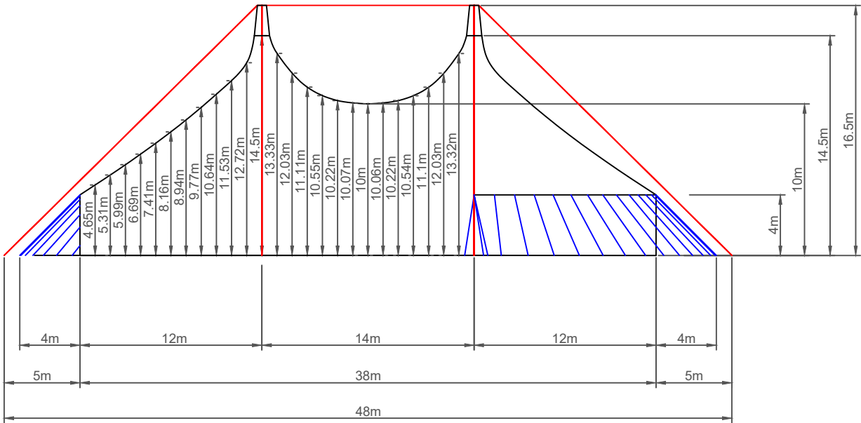
SIDE ELEVATION (NTS)
