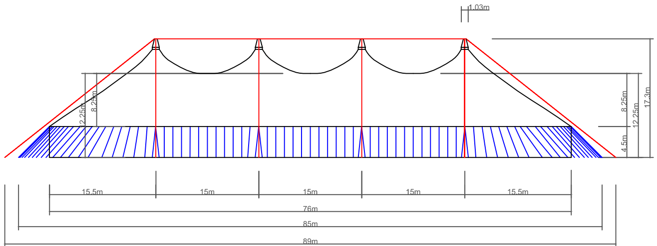
SIDE ELEVATION (NTS)
