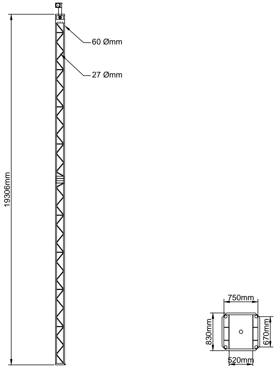
SUPPORT POLE & BASE PLATE DETAILS (NTS)
