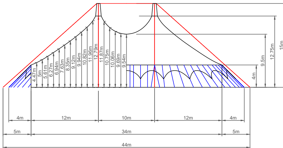
SIDE ELEVATION (NTS)
