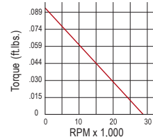
Torque-Speed Chart AM-310
