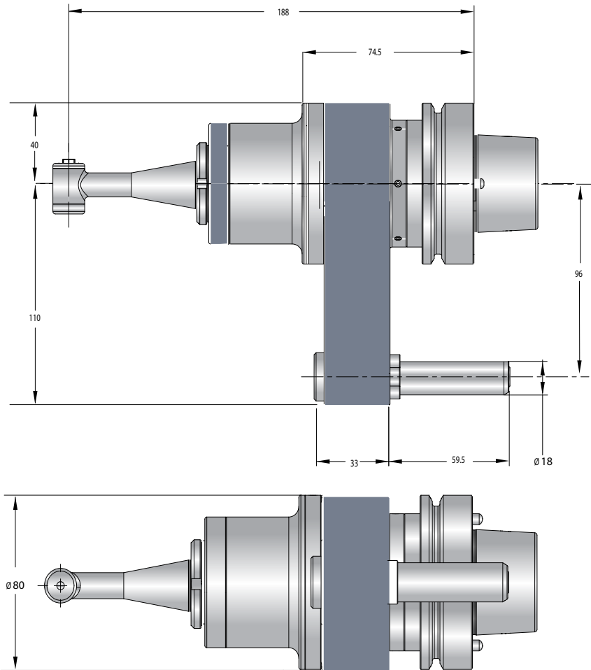
MAG1 Optional Programmable Spindle allows 360 degree positioning of the NSK output.
