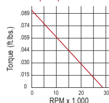
Torque-Speed Chart AM-310
