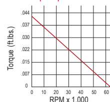
Torque-Speed Chart AM-600
